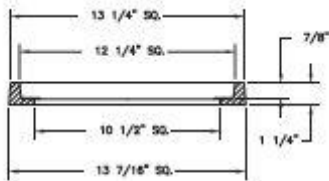
FRAME SECTION
